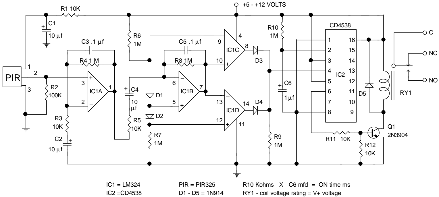
MOTION DETECTOR
